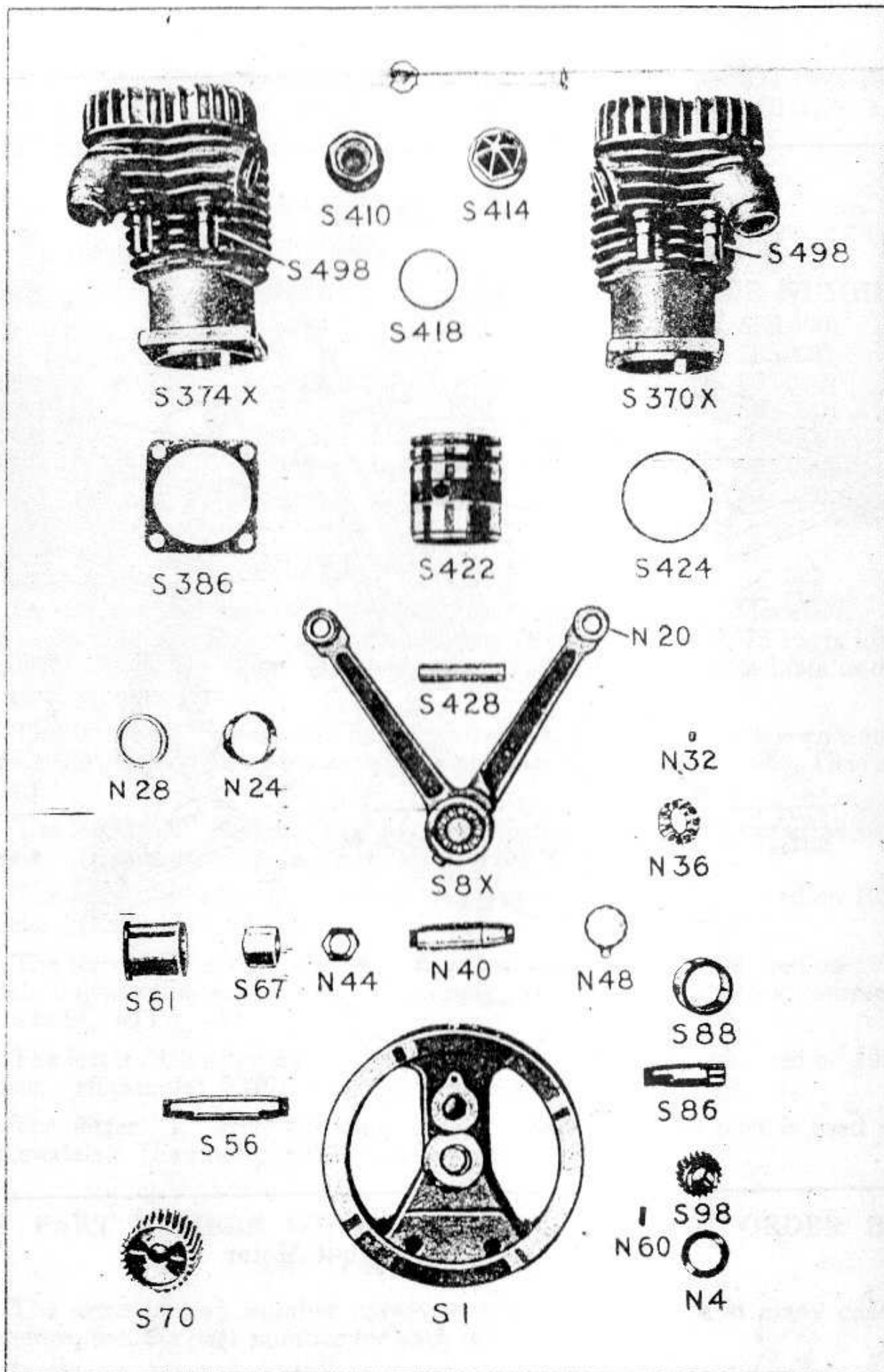
Fly Wheel and Crank Motion Group Cylinder and Piston Group
