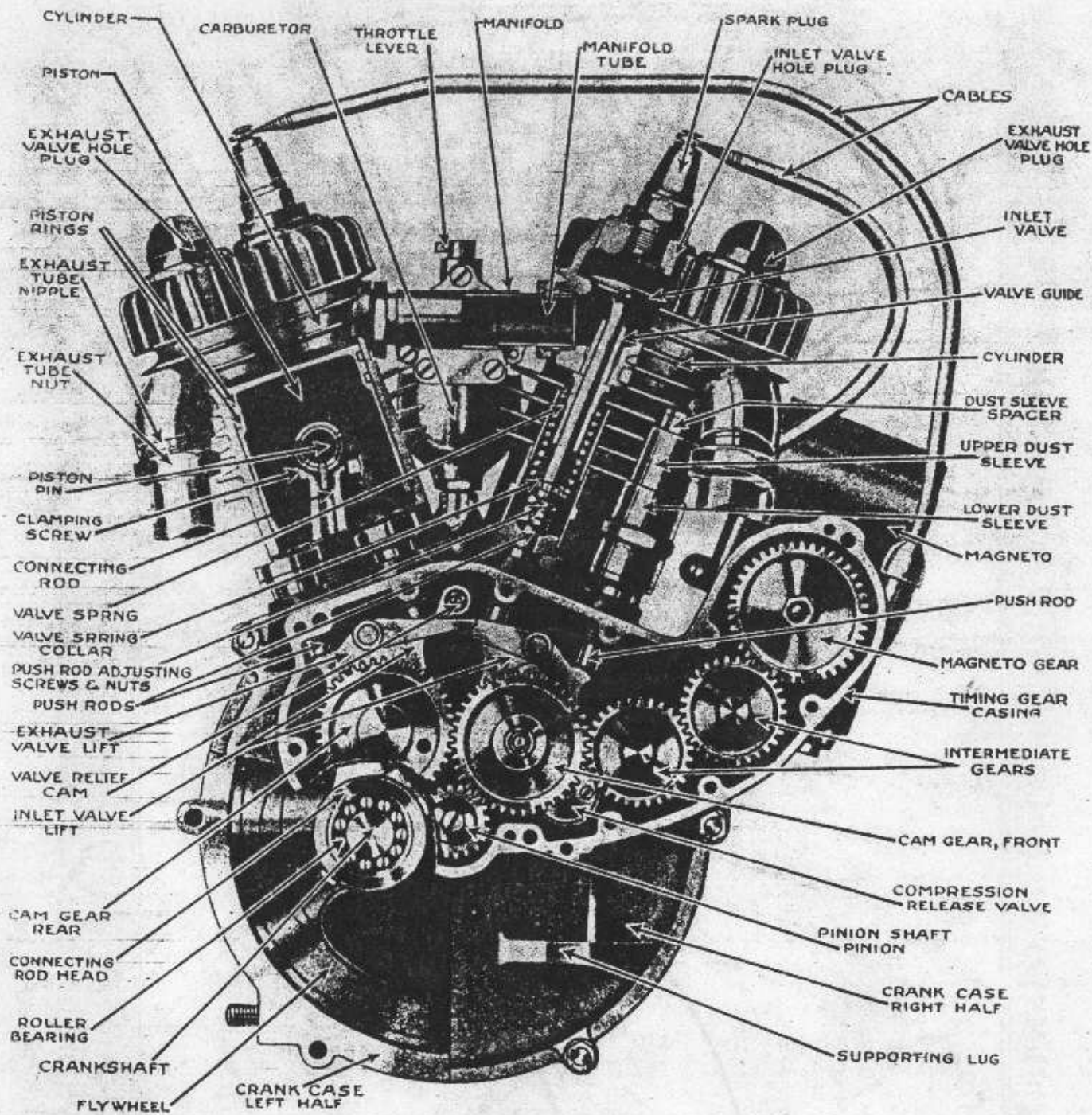
Sectional View G-20 Motor
