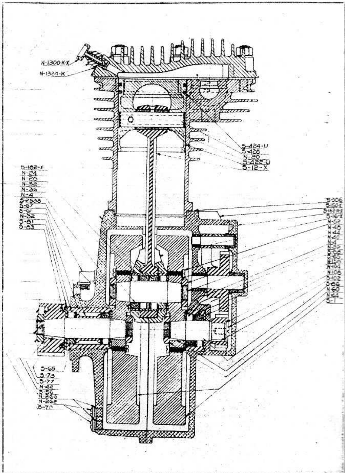
Sectional View 1926 Scout Motor
