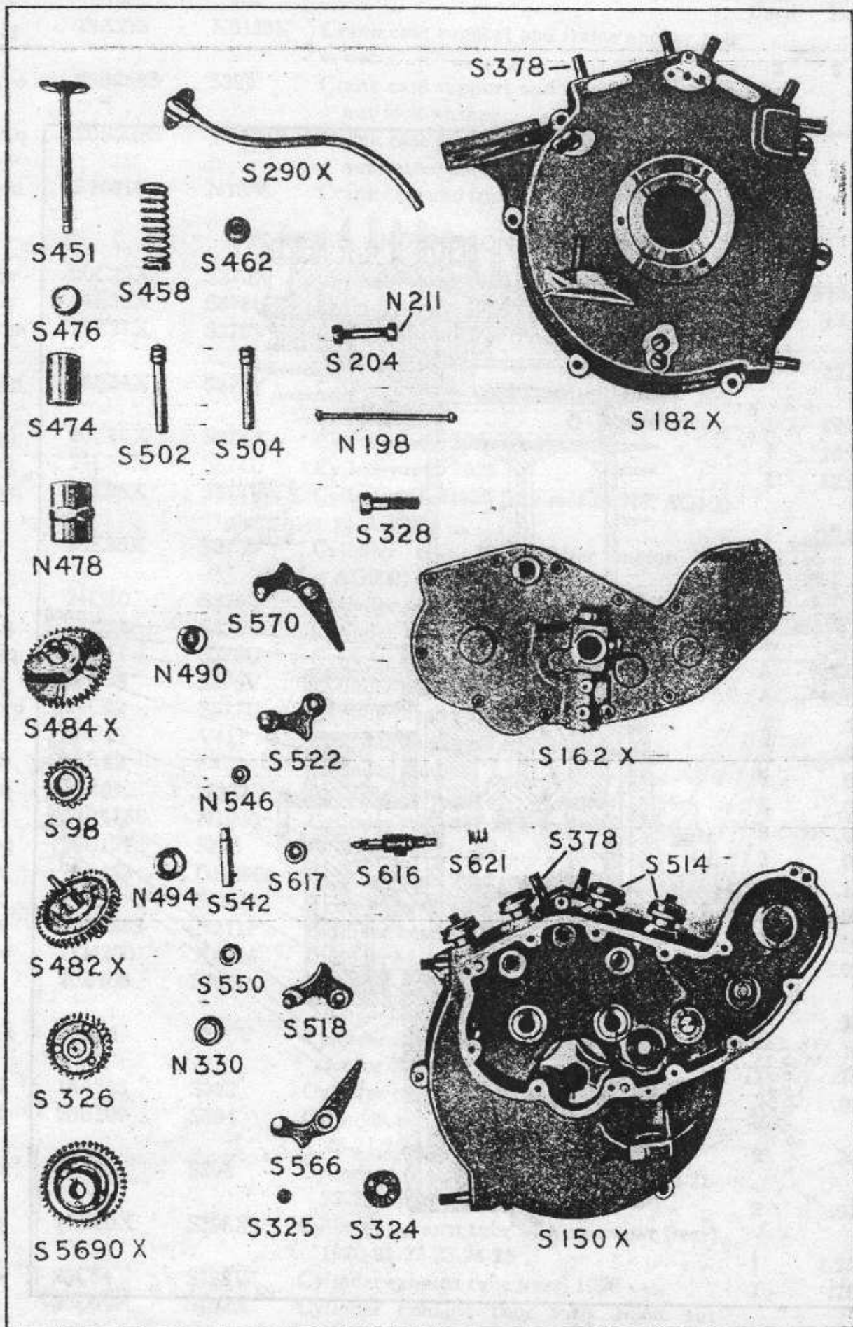
Crank Case and Valve Group 1920-1924
