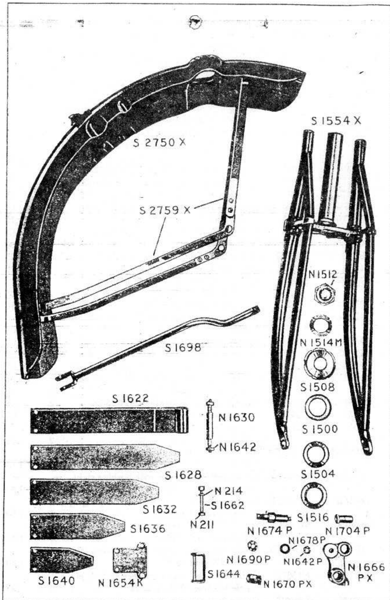
Fork Group Model G-20-21-22-23
