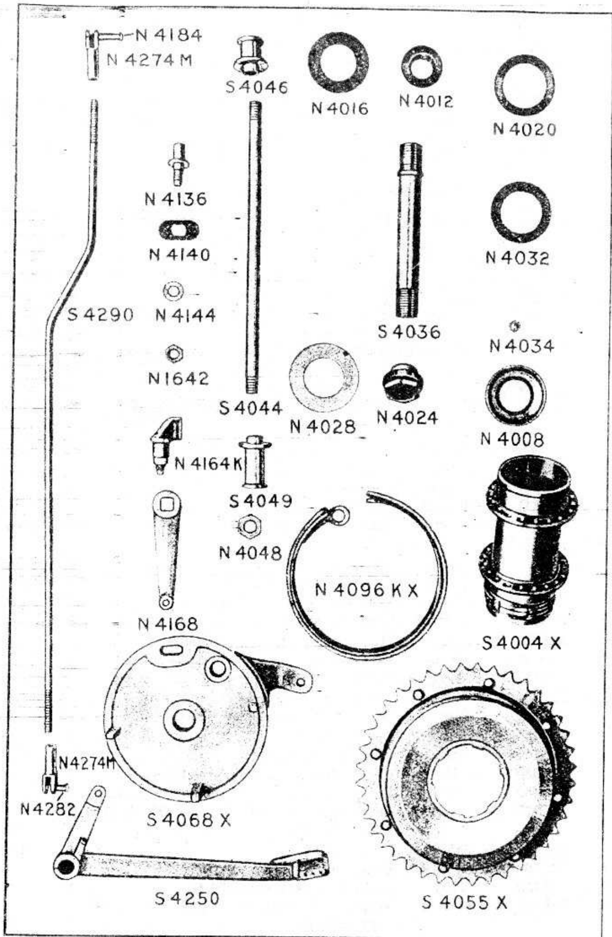
Rear Wheel and Brake Group
