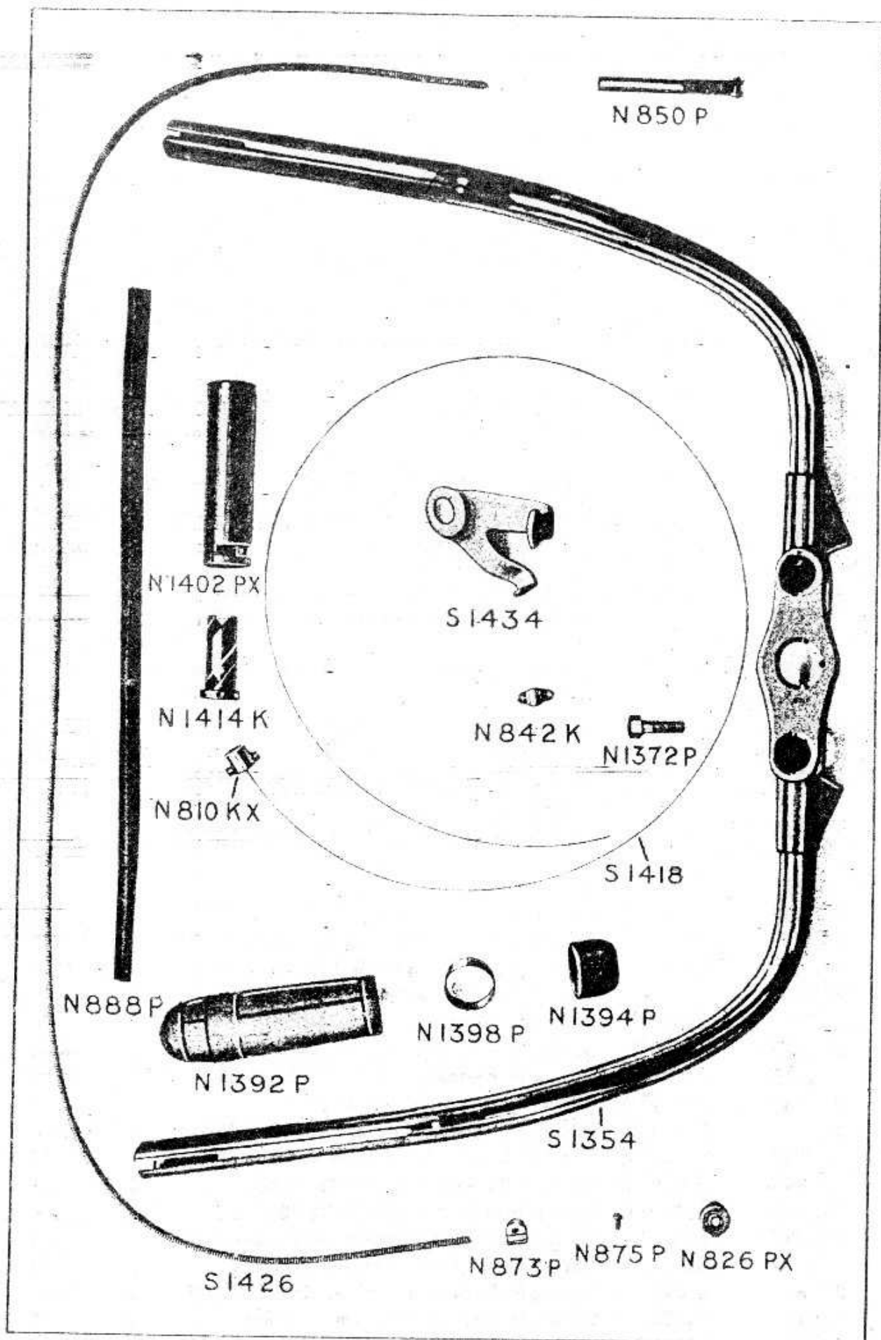
Handle Bar and Grip Control Group 1920-1924
