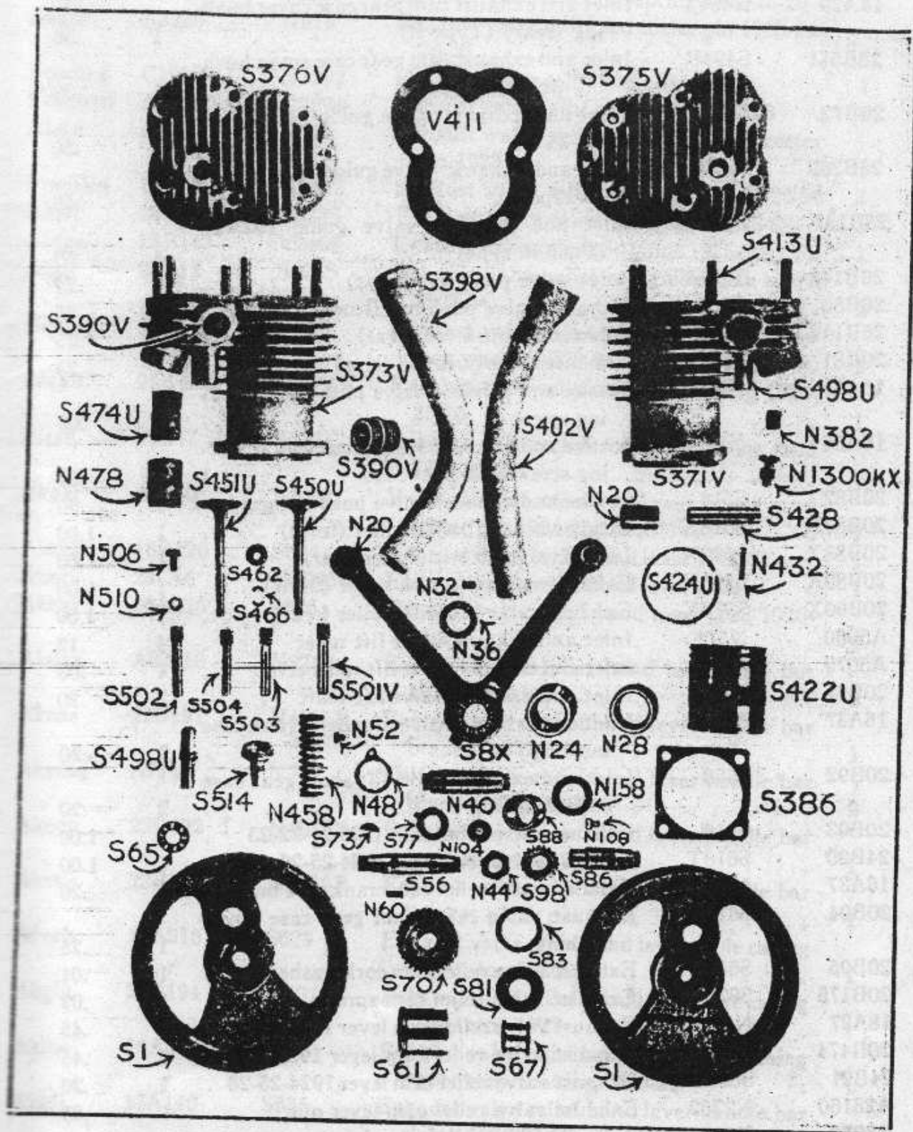
Crank Motion—Cylinder—Piston Groups 1926
