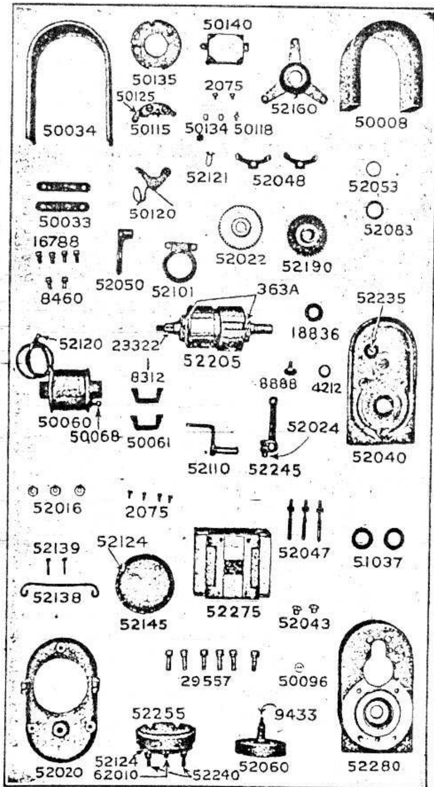
S-2 Magneto Group
