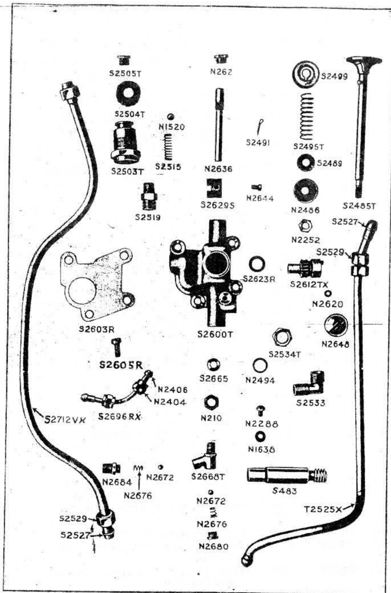
Automatic Oiler Group 1926
