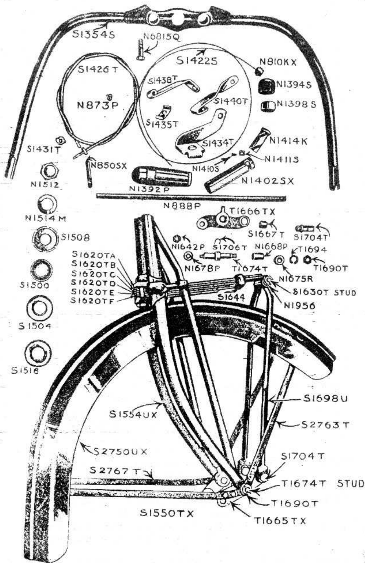
Handle Bar—Front Fork Groups 1926
