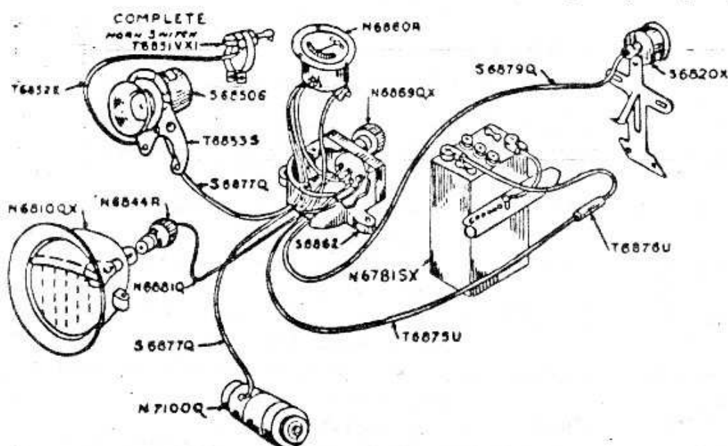
Wiring Diagram 1926
